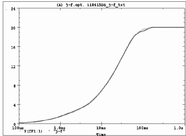
Si8415DB Filter j-f Temperature: 27.0
