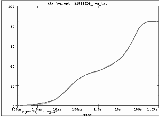
Si8415DB Tank j-a Temperature: 27.0
