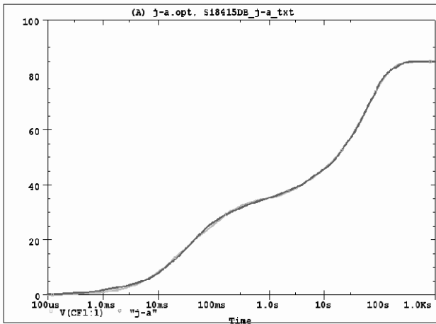
Si8415DB Filter j-a Temperature: 27.0
